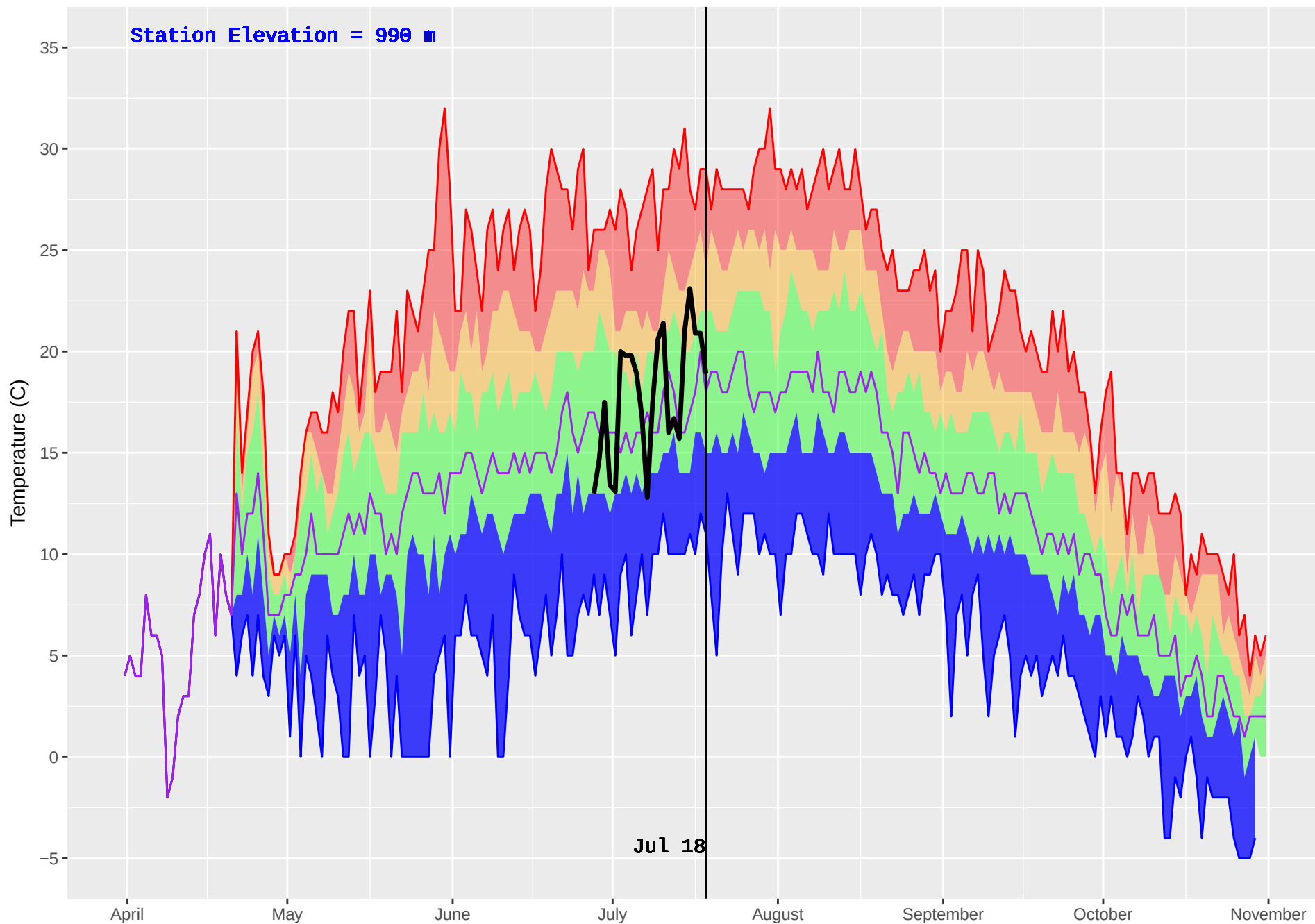
LOVELL COVE (163) : Historical (1979–2016) and Current (2018) Daily Temperature
